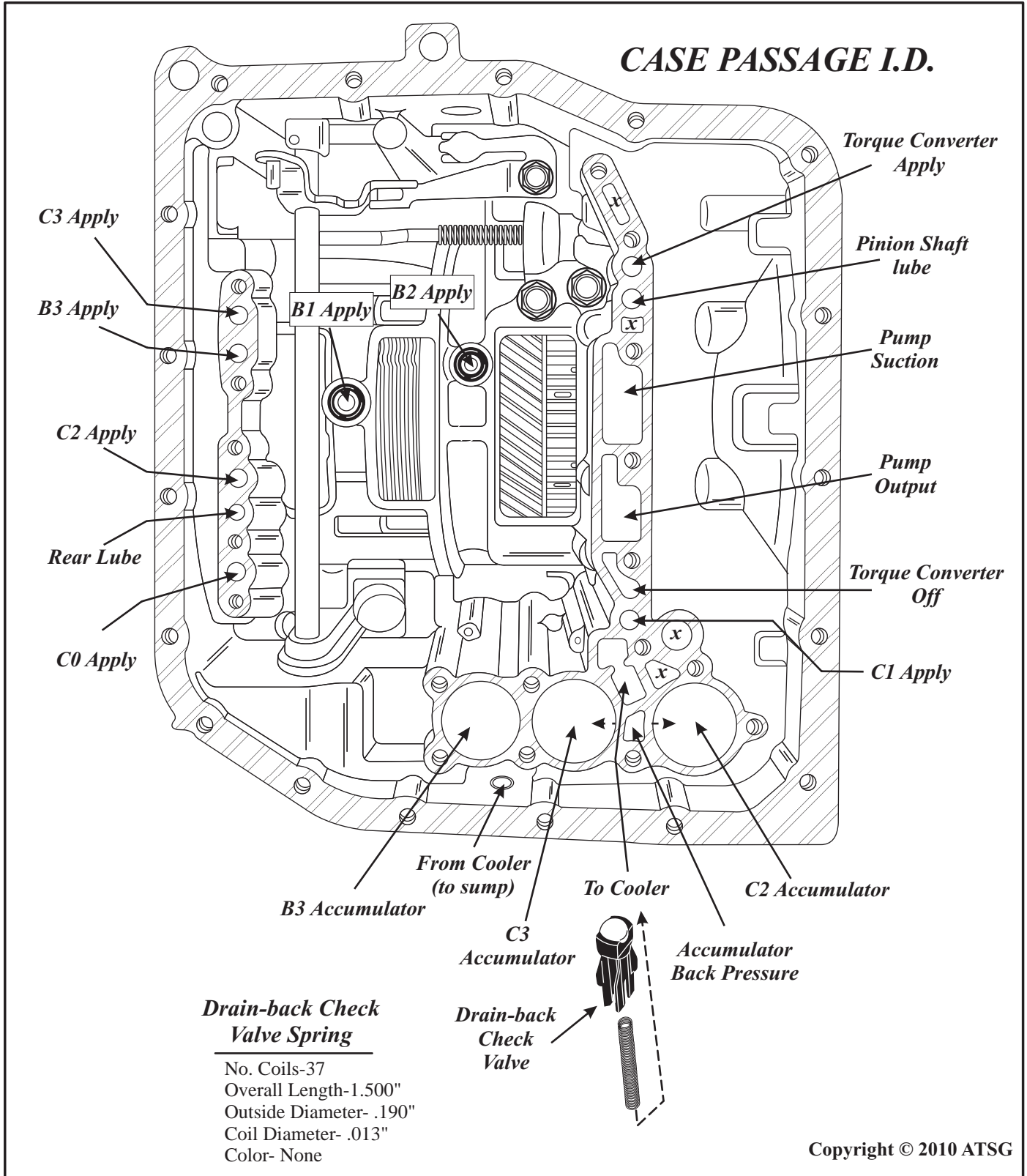
Figure 25 Automatic Transmission Service Group
